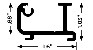
1" Extension Riser
