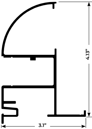
THREE-SIXTY-FIVE™ Coping
